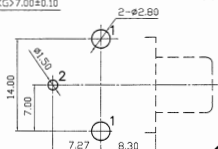
Pin Hole Layout (Jack Bottom View)
