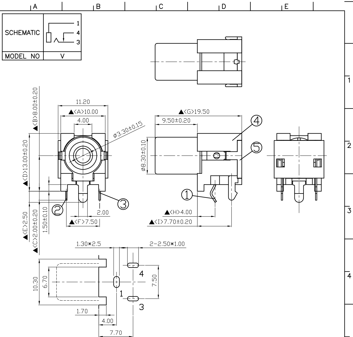
Pin Hole Layout (Jack Bottom View)
