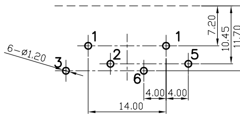
Pin Hole Layout (Jack Bottom View)
