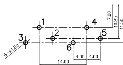
Pin Hole Layout (Jack Bottom View)
