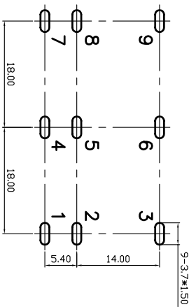
Pin Hole Layout (Jack Bottom View)
