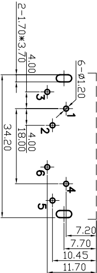
Pin Hole Layout (Jack Bottom View)
