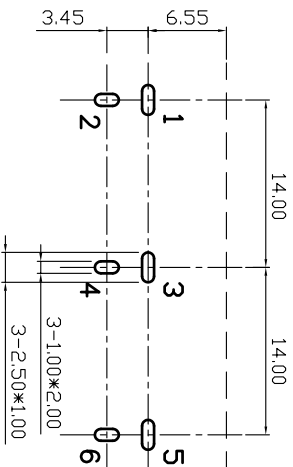
Pin Hole Layout (Jack Bottom View)
