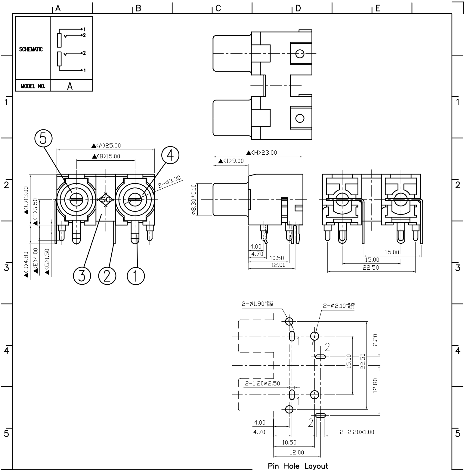
Pin Hole Layout (Jack Bottom View)
