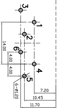
Pin Hole Layout Jack Bottom View
