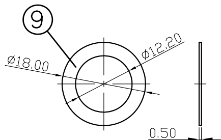
WASHER
