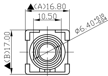
M12XP1.0 METRIC THREAD
