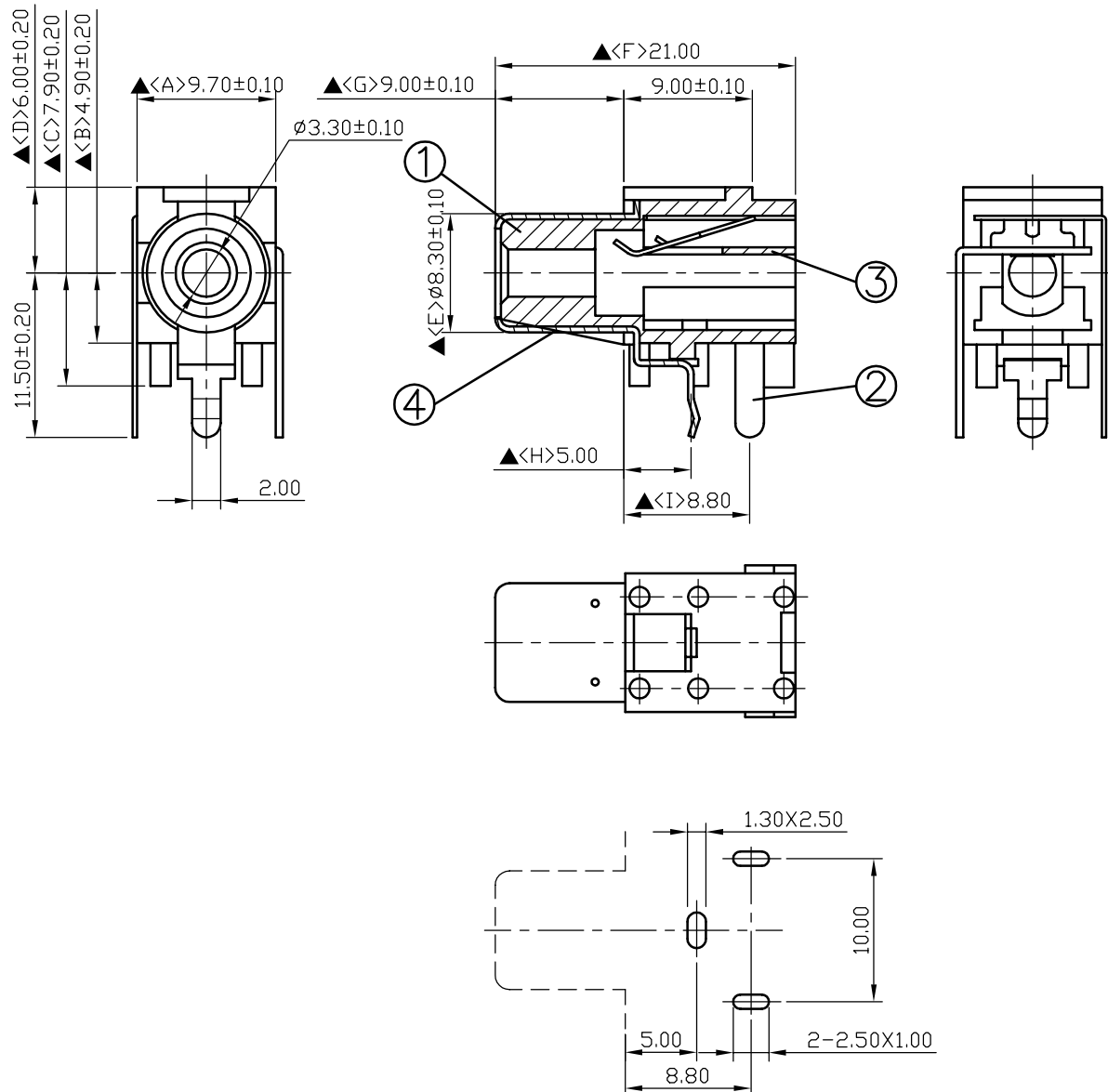
Pin Hole Layout (Jack Bottom View)
