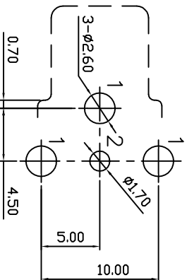
Pin Hole Layout (Jack Bottom View)
