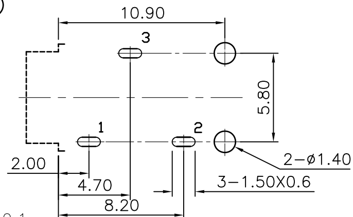
Pin Hole Layout (Jack Bottom View)
