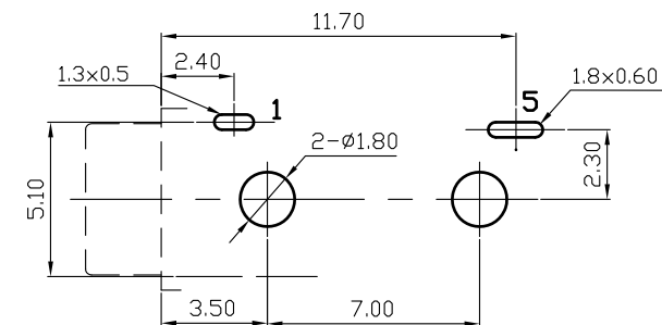
Pin Hole Layout (Jack Bottom View)
