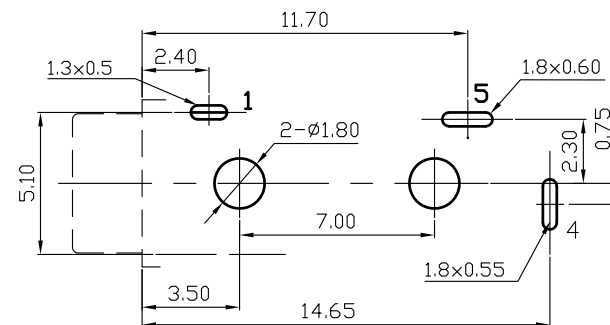
Pin Hole Layout (Jack Bottom View)
