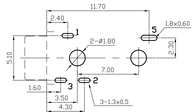
Pin Hole Layout (Jack Bottom View)
