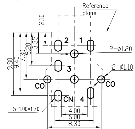
Pin Hole Layout (Jack Bottom View)
