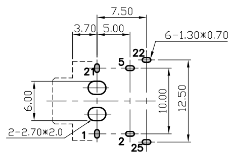
Pin Hole Layout (Jack Bottom View)
