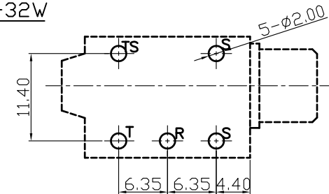
Pin Hole Layout (Jack Bottom View)
