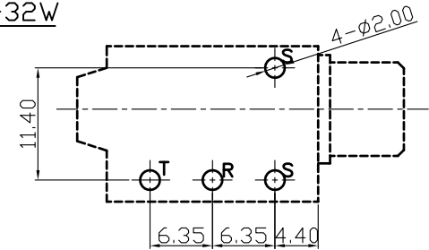
Pin Hole Layout (Jack Bottom View)
