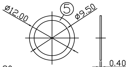
WASHER
