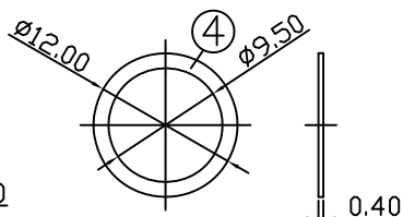
WASHER
