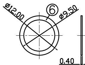
WASHER
