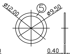
WASHER
