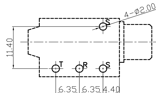
Pin Hole Layout (Jack Bottom View)
