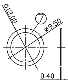
WASHER
