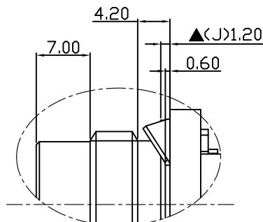
"A"Detail
