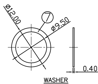
WASHER
