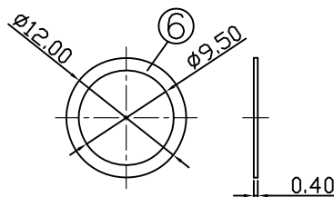
WASHER
