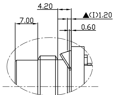
"A"Detail
