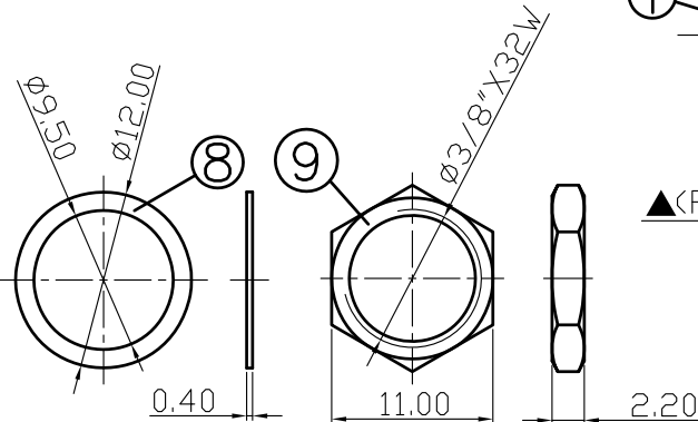
WASHER
