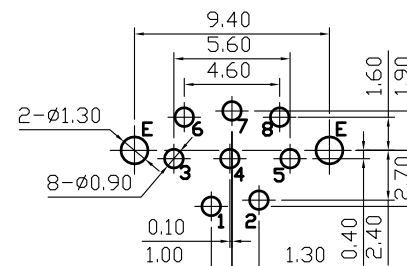
Pin Hole Layout (Jack Bottom View)
