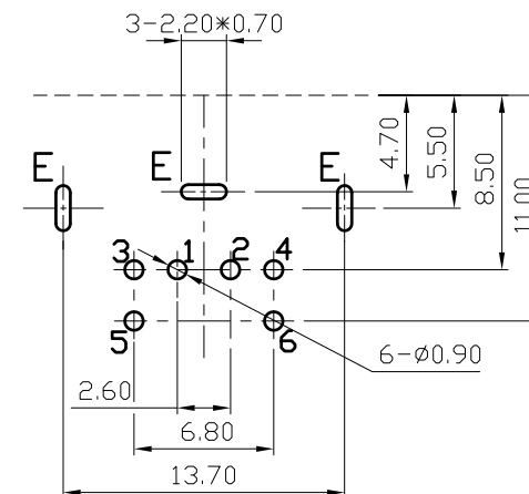
Pin Hole Layout (Jack Bottom View)
