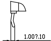
DETAIL "A"(1:1)
