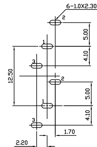
PIN HOLE LAYOUT JACK BOTTOM VIEW
