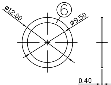
WASHER
