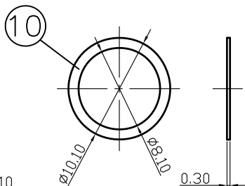
WASHER
