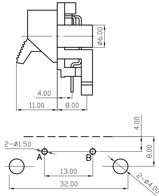
Pin Hole Layout (Jack Bottom View)
