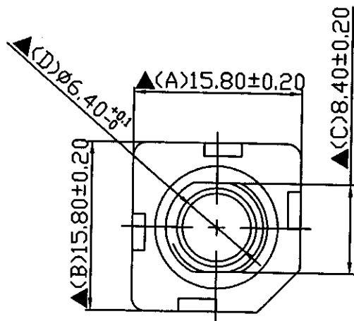
3/8"X32W PLASTIC BUSHING
