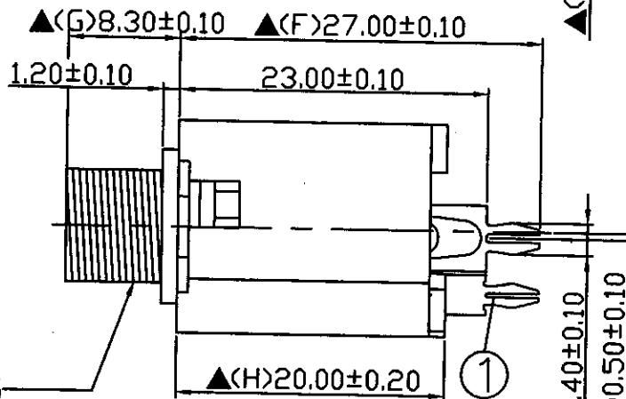
3/8"X32W PLASTIC BUSHING
