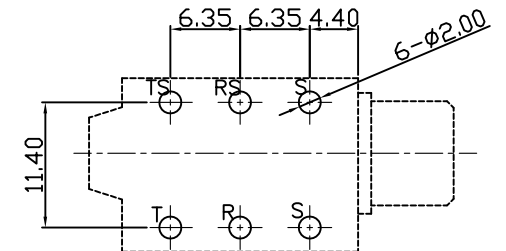
Pin Hole Layout (Jack Bottom View)
