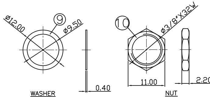
WASHER
