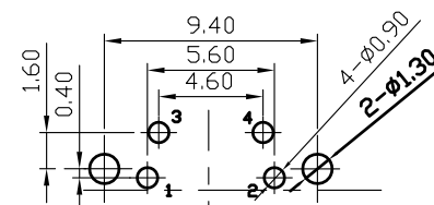
Pin Hole Layout (Jack Bottom View)
