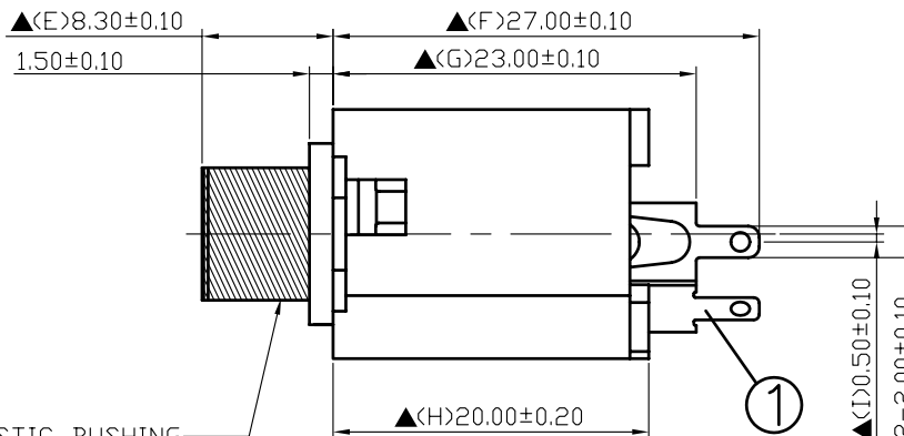
\phi 3/8'' \times 32W PLASTIC BUSHING
