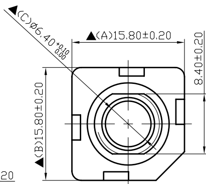
\phi 3/8'' \times 32W PLASTIC BUSHING
