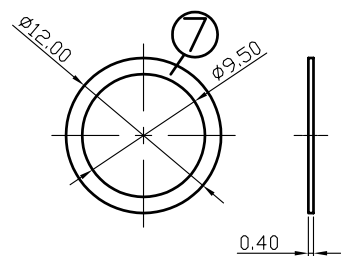
WASHER
