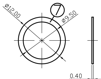
WASHER
