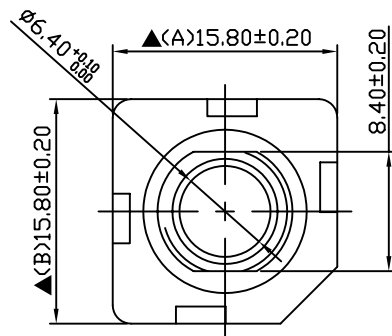
\phi 3/8 \times 32W PLASTIC BUSHING
