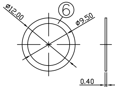
WASHER
