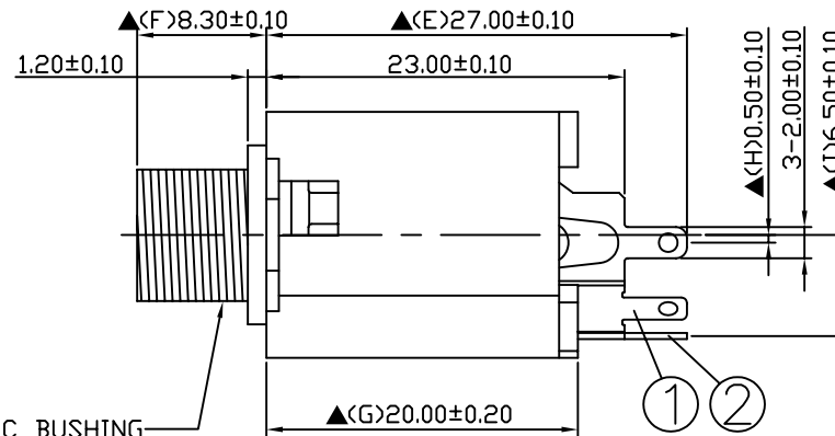
\phi 3/8 \times 32W PLASTIC BUSHING
