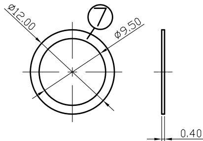
WASHER
