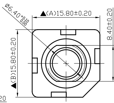
3/8"X32W PLASTIC BUSHING
