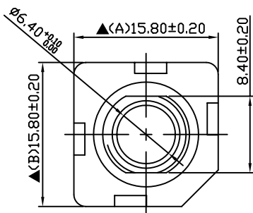
\phi 3/8 \times 32W PLASTIC BUSHING
