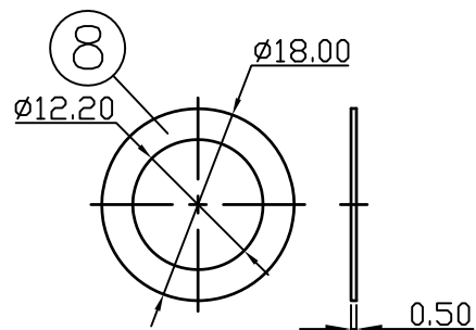
WASHER
