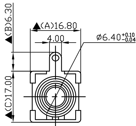
WASHER
