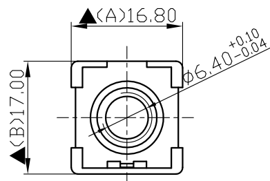
M9XP0.75 METRIC THREAD WITH STOPPER
