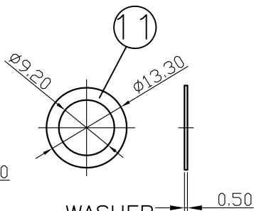
WASHER
