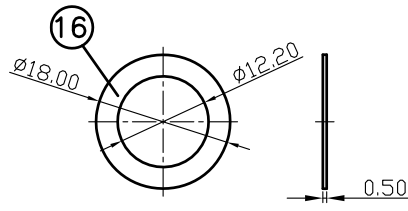
WASHER
