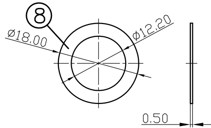
WASHER
