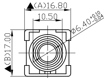
M12XP1.0 METRIC THREAD
